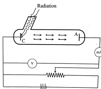
Figure 1: Experimental arrangement for photoelectric effect
